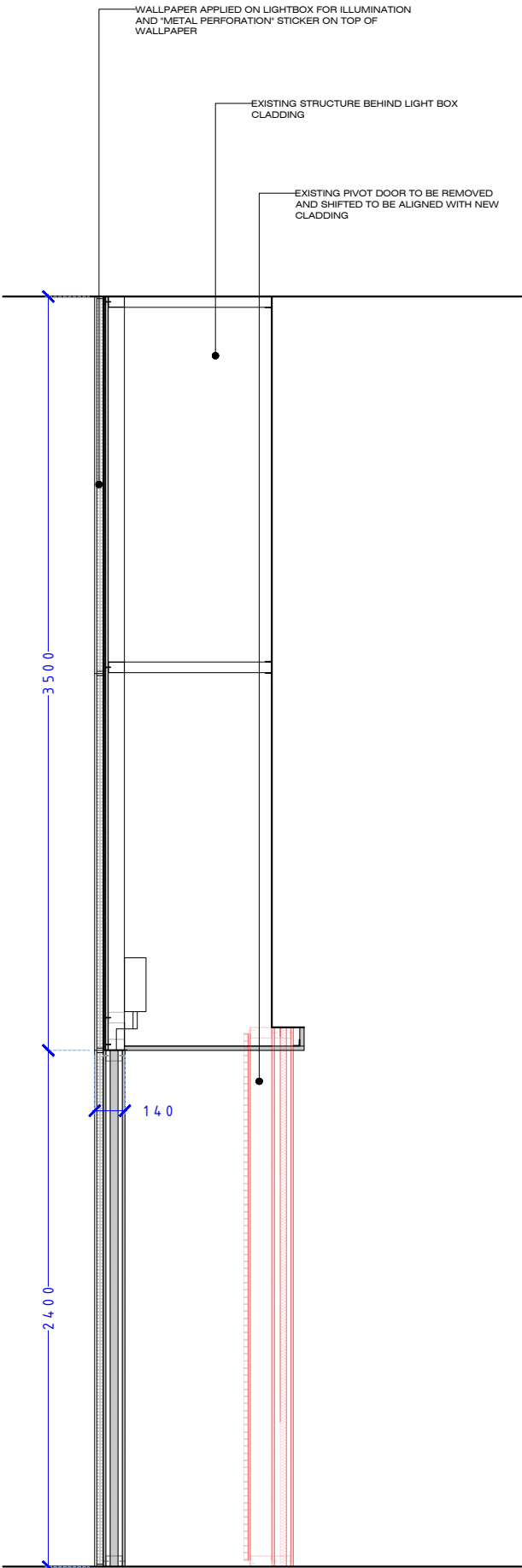
SIDE SECTION SCALE 1:30
