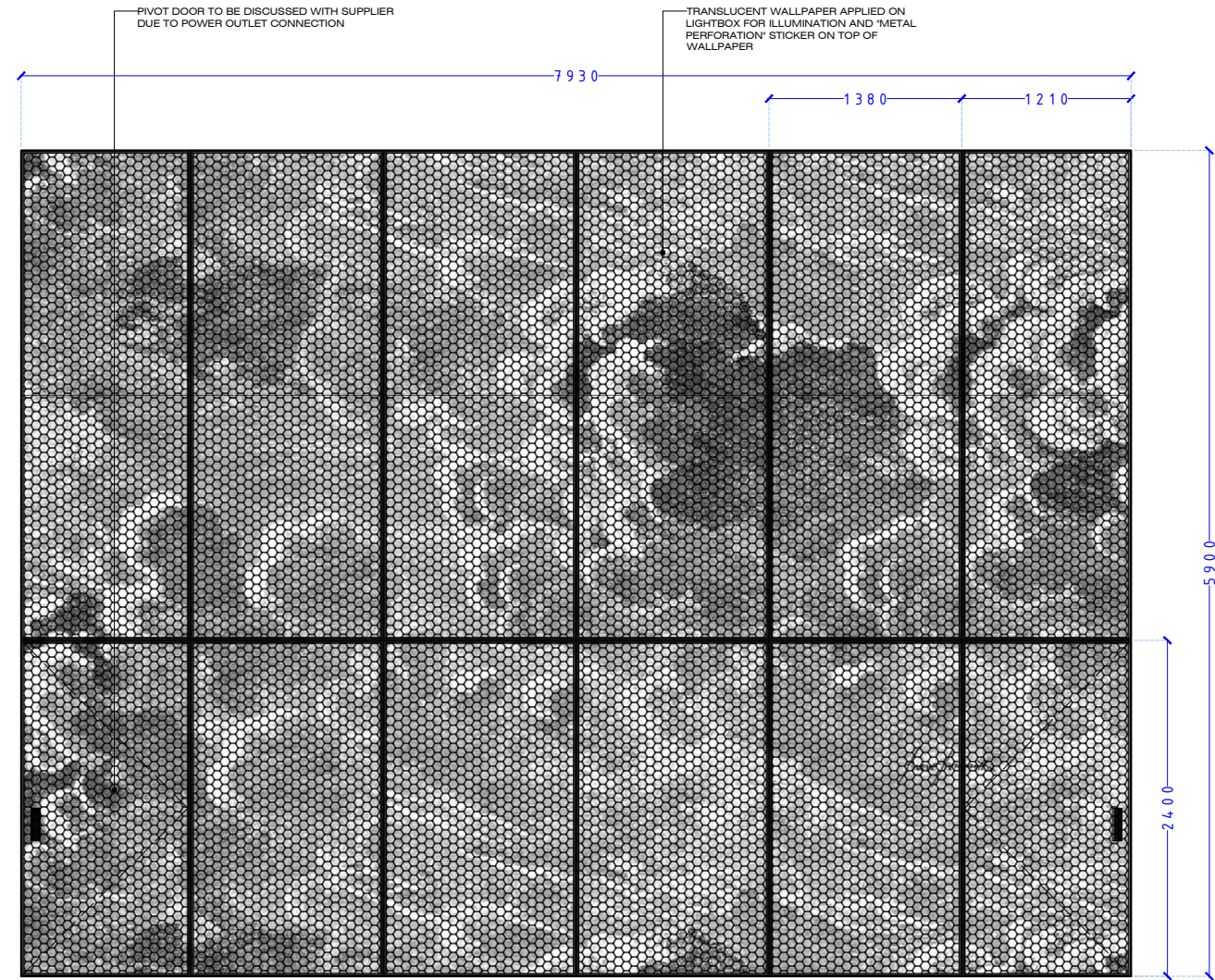
ELEVATION SCALE 1:50
